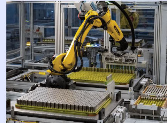
Cell placement
